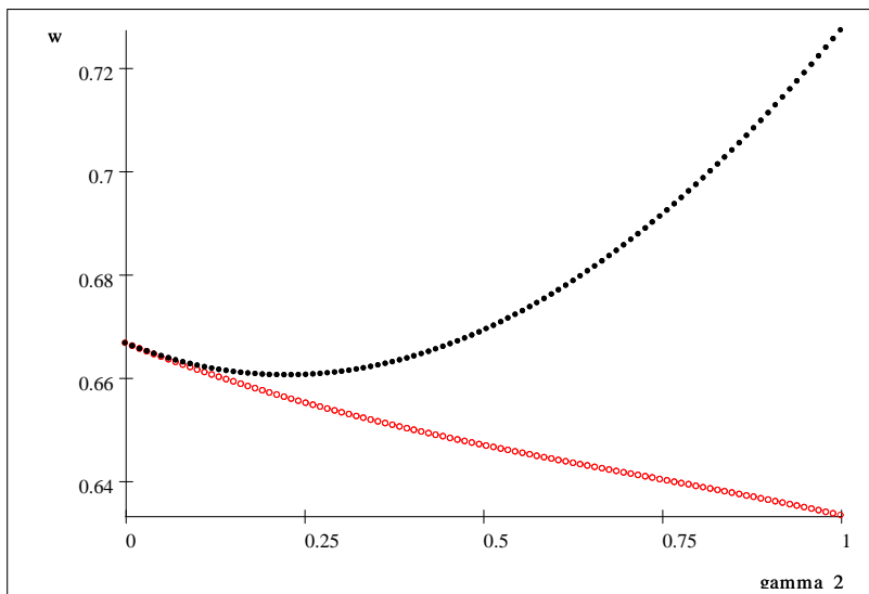
Figure 2. w_2^B : black dots, w_{2B}^B : red circles.
