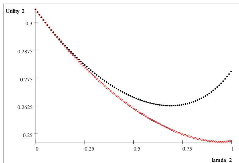
Figure 18. V_2^C : black dots, V_2^{Cmerger} : red circles.
